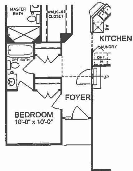
PARTIAL PLAN W/OPTIONAL FULL BATH AND OPTIONAL BEDROOM ONE LEVEL
