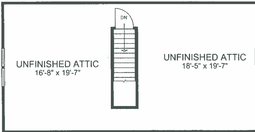
PARTIAL PLAN W/ OPT. UNFINISHED ATTIC
